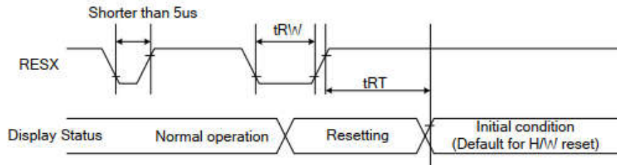
Figure 125: Reset Timing
